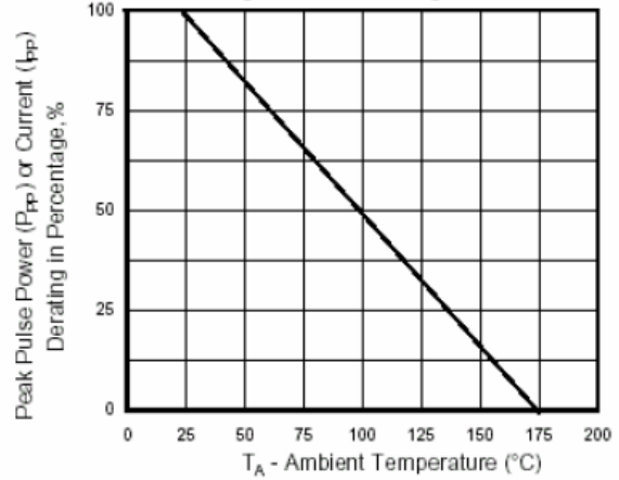
Fig.2-Power Derating Curve
